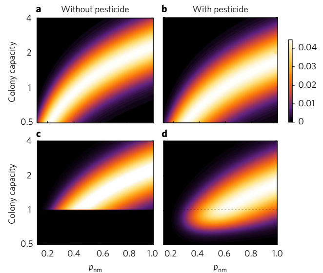
Fig. 3 | Effect of pesticide exposure on colony capacity. a–d, Heat maps showing the likelihood profiles for the colony capacity taking certain values without (a,c) or with thiamethoxam exposure (b,d). Each heat map represents the probability distribution (normalized likelihood) of the colony capacity (where lighter colours indicate a higher probability; see the scale to right of the graphs) as a function of p_{nm} and the colony capacity itself. The colony capacity is the multiplication of p_{nm} with the number of gynes produced 51 , the probability of surviving hibernation 45 and the probability of being able to initiate a colony following survival. a, Probability that the colony capacity takes a certain value for different values of p_{nm} (using data from 45,52 ). b, Likelihood profile of the colony capacity after exposure to thiamethoxam; the distribution is lower than in a due to the reduction in colony initiation (as found in our empirical results; see Supplementary Material for methodology). c, Likelihood profile of the colony capacity without exposure to thiamethoxam, conditioned to take a value of at least 1 to take account for the natural bumblebee population of B. terrestris being extant. The colony capacity must therefore be at least 1. The likelihoods for the colony capacities below 1 were therefore set to 0 and the profile was re-normalized. d, Likelihood profile for the colony capacity as in c after the effect of thiamethoxam exposure was taken into account. Because of the reduction in colony initiation caused by thiamethoxam exposure, colony capacities below 1 have positive probability. The total probability of a colony capacity below 1 is found by integrating all probabilities below the dashed line in d.
