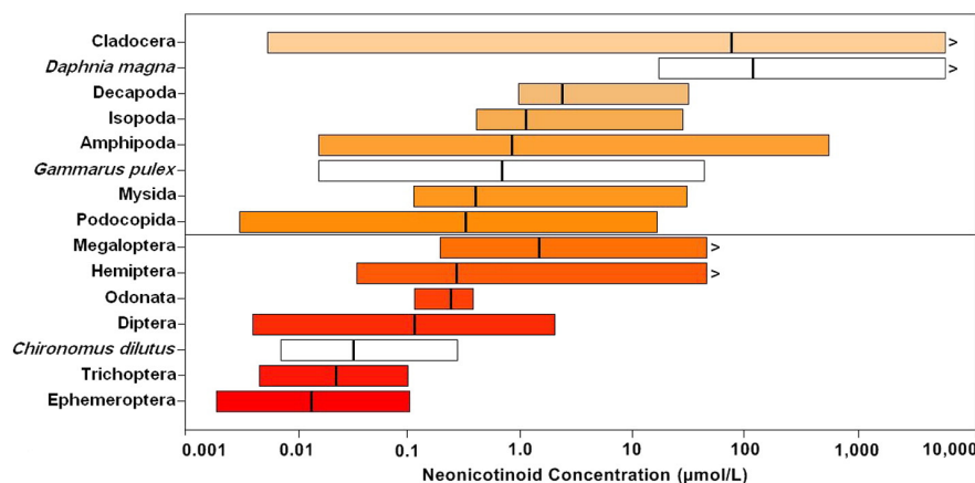
Fig. 2. Range of neonicotinoid toxicity (L[E]C 50 : 24–96 h in \mu\text{mol/L} ) among all tested aquatic invertebrate orders. For context, three of the most common test species (open bars) for the orders Cladocera ( Daphnia magna ), Amphipoda ( Gammarus pulex ) and Diptera ( Chironomus dilutus ) are shown to illustrate differences in sensitivity by species. Vertical lines within bars represent geometric means of test values (see also Table 2).
