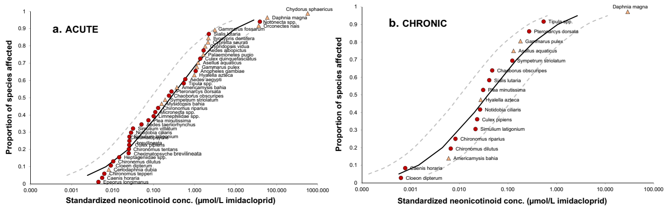
Fig. 5. Species sensitivity distributions for a) 137 acute ( \text{LC}_{50} : 24–96 h) laboratory toxicity tests with 42 different aquatic invertebrate species, and b) 36 chronic ( [\text{E}]\text{C}_{50} : 7–39 day) laboratory toxicity studies with 18 aquatic invertebrate species. Red circles represent aquatic insects and orange triangles represent crustaceans. Distributions are based on test values of multiple neonicotinoid compounds with concentrations standardized to imidacloprid molecular mass. (For interpretation of the references to color in this figure legend, the reader is referred to the web version of this article.)
