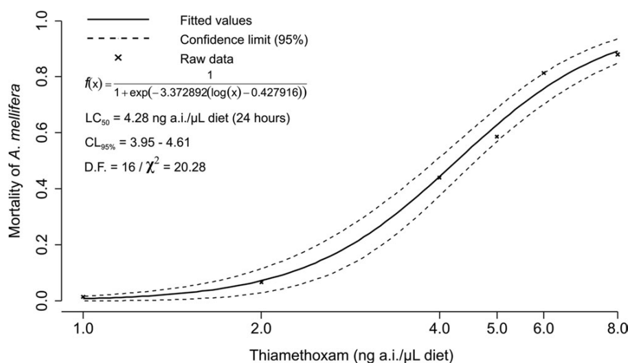
Fig. 1. Mortality of newly emerged workers of Africanized A. mellifera according to the ingestion of food contaminated with several doses of thiamethoxam (1–8 ng/ \mu L diet).
