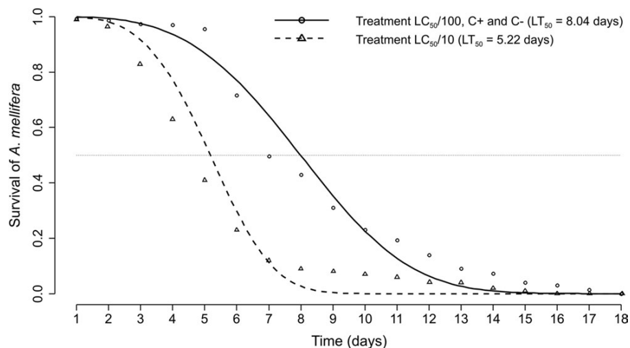
Fig. 2. Survival rate of newly emerged workers of Africanized A. mellifera according to the food intake during different treatments: control without solvent (C - ); solvent control (C + ); 1/10 of LC 50 of thiamethoxam (0.428 ng i.a./ \mu L diet) and 1/100 of LC 50 of thiamethoxam (0.0428 ng i.a./ \mu L diet).
